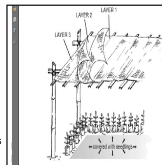
FIGURE 2. A SAMPLE HARDENING BED.
